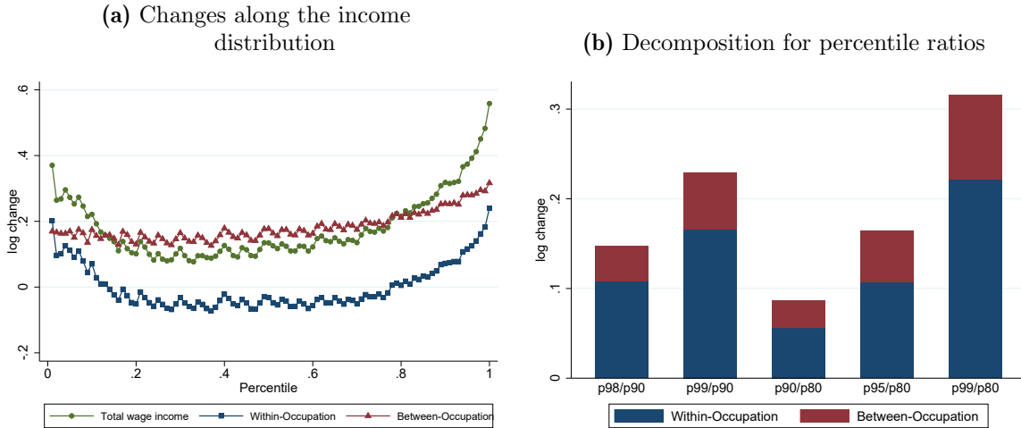
Figure 1: Changes in wage income from 1980 to 2012 - between and within occupations
