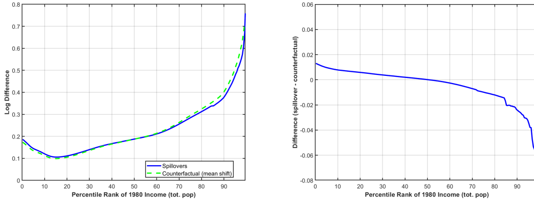
Figure E.4: Differences in welfare for full income distribution (with and without spillovers) (a) Welfare differences - spillovers and counterfactual (b) Difference between spillovers and counterfactual
