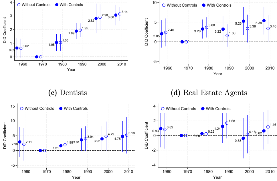
Figure 4: Finance Deregulation Reduced Form (a) First Stage (b) Physicians
