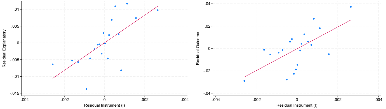
Figure D.1: Graphical Representation of the IV regression: residual top income inequality. (a) (First Stage) Top income inequality vs. instrument (b) (Reduced Form) Physician top income inequality vs. instrument
