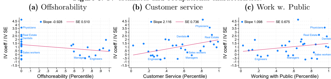
Figure 3: IV estimates and occupational characteristics.
