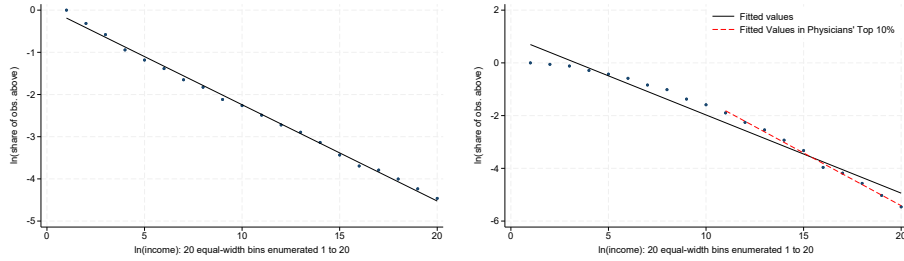
Figure 2: Fit of the Pareto Distribution - New York State (2000) (a) All Occupations (b) Physicians
