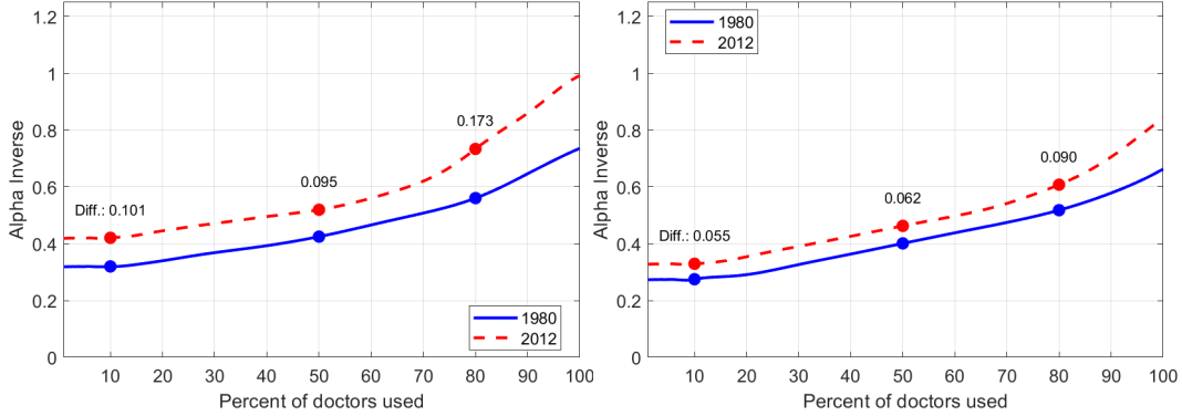
Figure B.1: Estimated \alpha^{-1} for doctors for various cutoffs. (a) New York State (b) National
