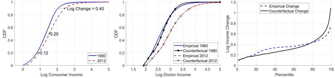
Figure 5: CDFs of income for consumers and physicians in New York State (a) Consumer income distribution (b) Doctor income distribution (c) Change in Doctors income
