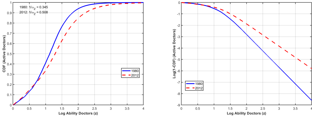
Figure E.2: Calibrated doctor ability distribution (a) CDF (b) Pareto plot
